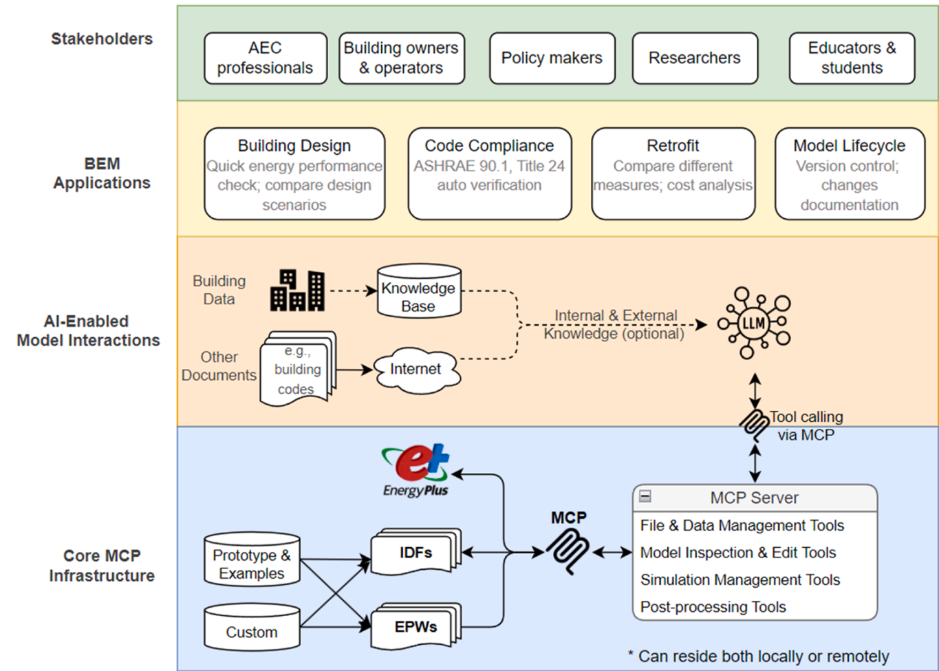
Fig. 2. EnergyPlus-MCP's role in the BEM ecosystem.
